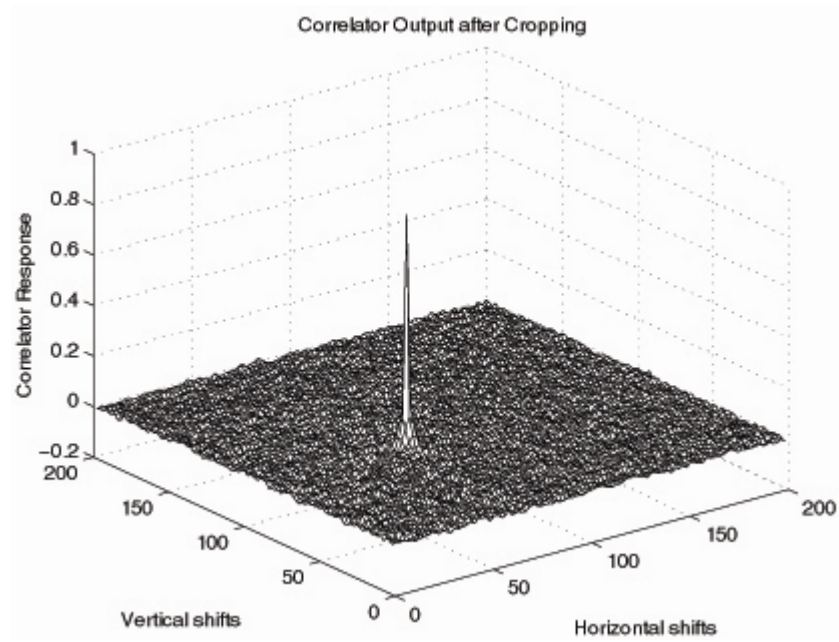
Fig. 12. Corellator response after cropping, cropped region [130:950, 90:930]
