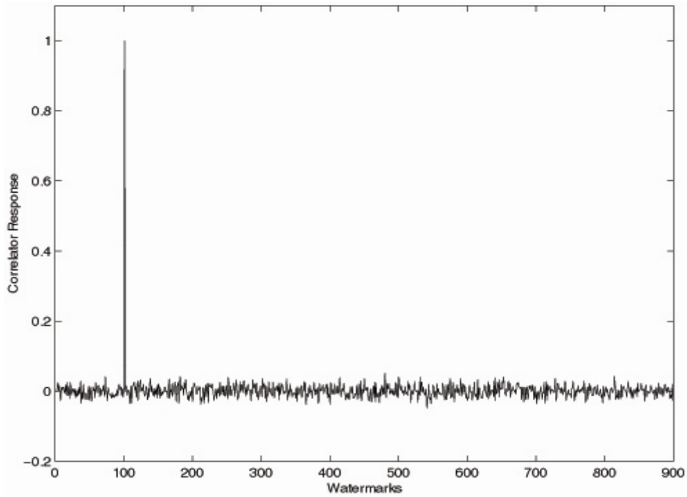
Fig. 6. Correlator response between 900 different watermarks and watermark no 100
